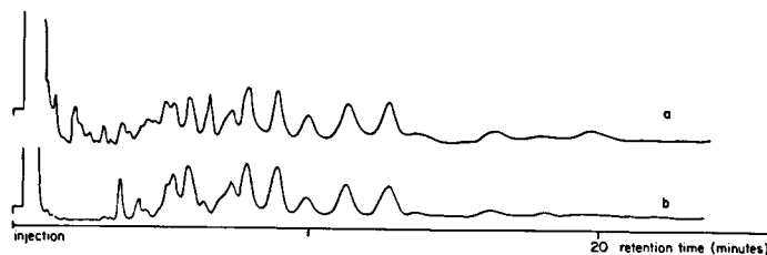
Fig. 3. Isothermal packed column chromatograms of same open ocean sample as in Fig. 2 (a) and Aroclor 1254 (b); column and conditions as in Fig. 1.
